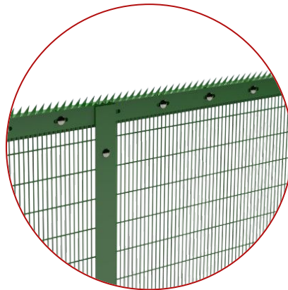
Wall Spikes Option B
